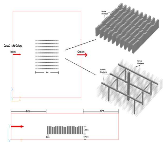
Figure 1 - CFD domain dimensions and zoomed in view of reefs (replaced with porous blockages) with and without support structures.
