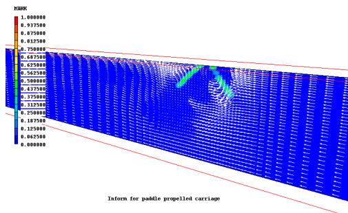
Figure 4. Snap shot of the flow showing paddles and velocity vectors.
