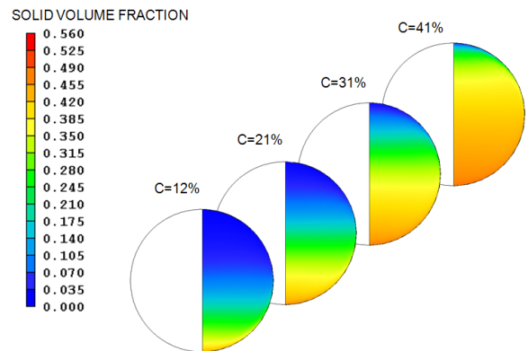
Figure 2 Contour plots for particle volume fraction
