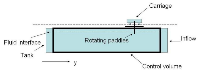
Figure 2. Control volume for momentum balance. An inflow equal to the carriage velocity has been applied on the North boundary tank face. On the opposite South tank wall a hydrostatic pressure outflow condition has been set.
