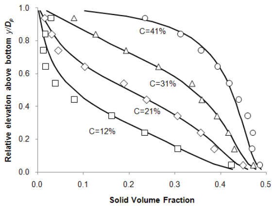
Figure 3 Particle concentration profiles: comparison between numerical predictions & experimental data of Gillies et al. [4].
