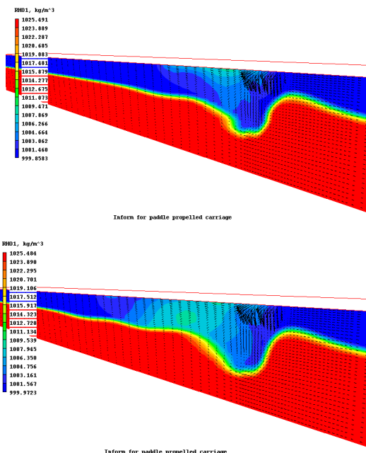
Figure 4. Snap shot of the flow showing paddles and velocity vectors.
