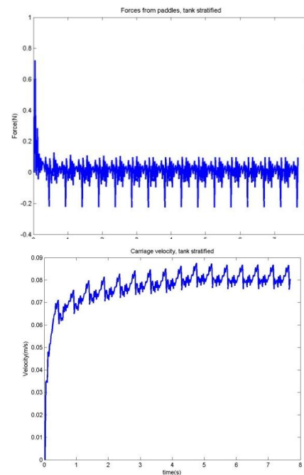
Figure 6. Top, force on carriage generated by paddles. Bottom, velocity of carriage.
