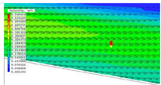
Figure 4 - Images of velocity flow contours with flow direction arrows with a) PARSOL off and b) PARSOL on
