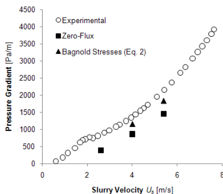
Figure 4. Pressure gradient versus slurry bulk-mean velocity: comparison between experimental data of Gillies et al. [4] & numerical predictions obtained using two boundary conditions
