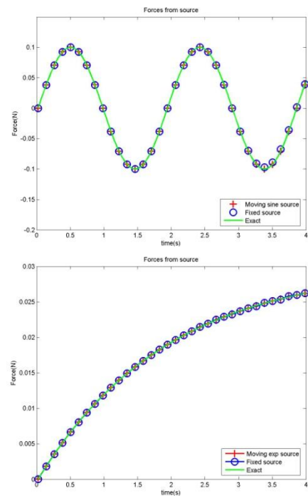
Figure 3. Top, sinusoid source. Bottom, exponential source. In each case simulations in stratified flow using INFORM have been conducted with the source moving and then with the source reduced to rest by applying the techniques described in the text.
