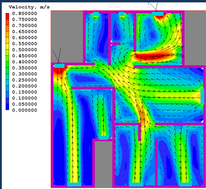
Figure 3 Velocity contours and vectors at z=1.45\text{m}
