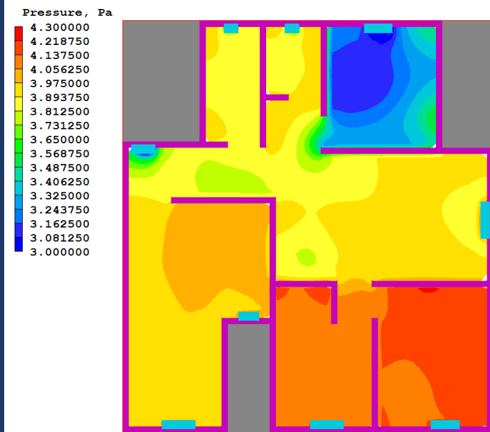
Figure 2 Pressure contours at z=1.45\text{m}
