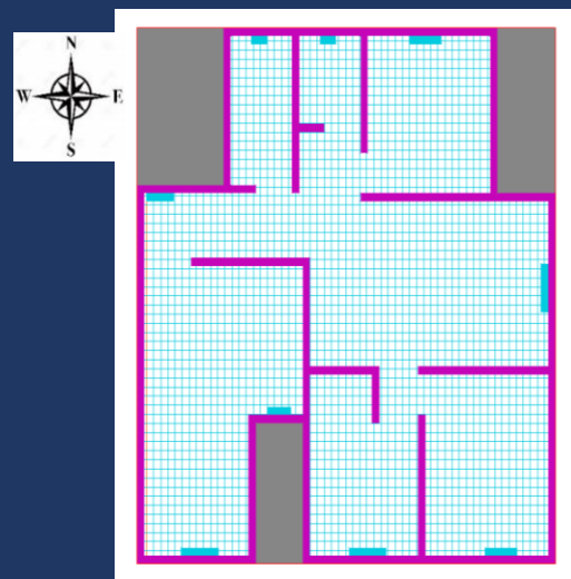
Figure 1 60 \times 60 \times 30 Cartesian mesh
