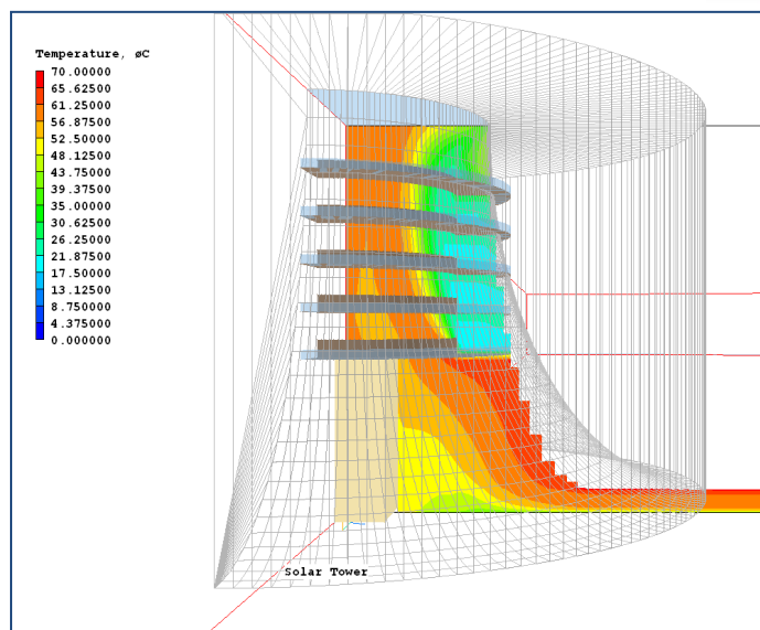
Temperature contours
