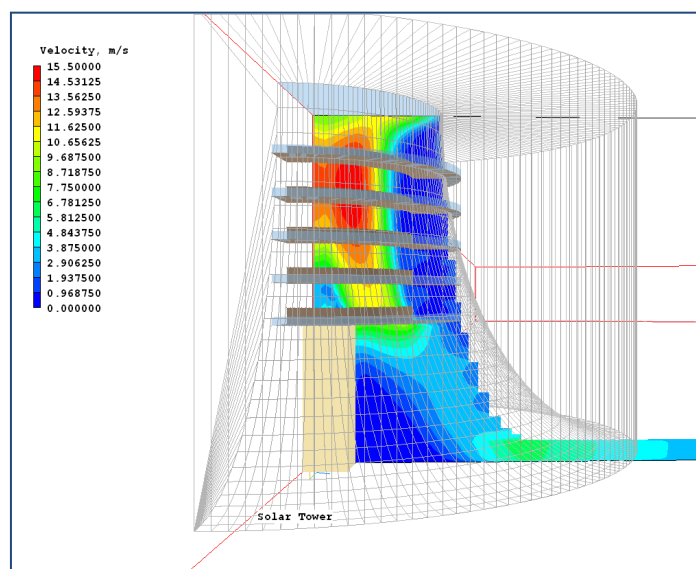
Velocity contours
