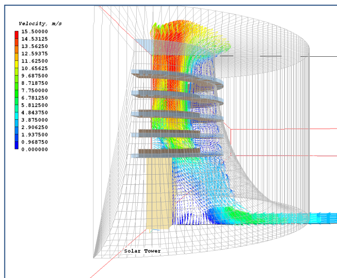
Velocity vectors
