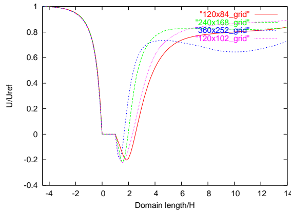
Fig. 7. The mean axial velocity distribution on the center plane of the cylinder from several simulations using different 2D grids
