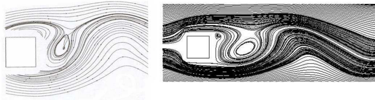
Fig. 10. Experimental and numerical streamlines
