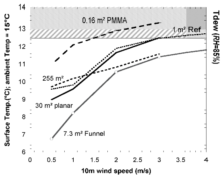
Fig. 6. Averaged surface temperatures obtained by numerical simulations and related to wind speed (10 m elevation). No condensation occurs in the gray area ( T_{cond} < T_d = 12.5 °C, RH < 85 %).
