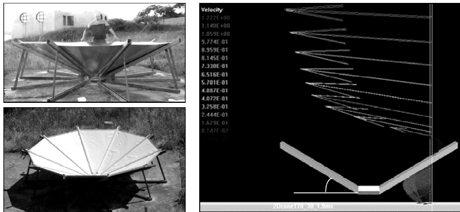
Fig. 3. Pictures of the funnel-shaped pilot (7.32 m 2 ) and its corresponding 2D simulation. The internal surface is coated with OPUR Low Density PolyEthylene film insulated from below with 3 cm Styrofoam.
