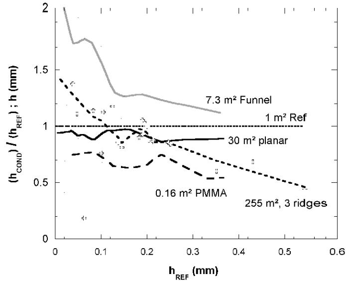
Fig. 8. Measurements of dew yields (mm/night) for all 5 condensers with respect to the planar 1 m 2 condenser. Data are smoothed by a 40% weighing function to enlight tendencies. Crosses represent the yields as measured on one ridge of the dew plant.
