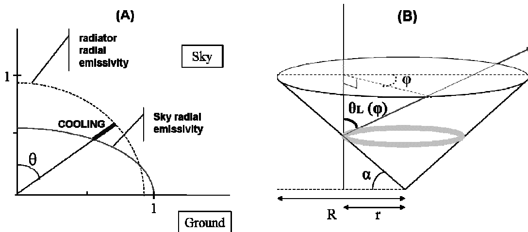
Fig. 1. (a) Variation of both radiator and sky emissivities with respect to the inclination angle \theta (degree) with vertical. The bold line represents the neat cooling power (see text). (b) Integration performed for a funnel shape, from \theta = 0 to \theta = \theta_L ( \theta limit), from \varphi = 0 to \varphi = 360^\circ , from r = 0 to r = R . The result is weighted according to the surface of each funnel fraction (gray) with respect to the total funnel surface.
