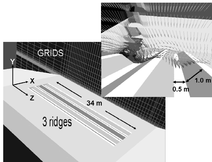
Fig. 2. Overview and detail of three ridges (255 m 2 ) of the large scale condenser (India) as modeled in the virtual reality PHOENICS viewer.
